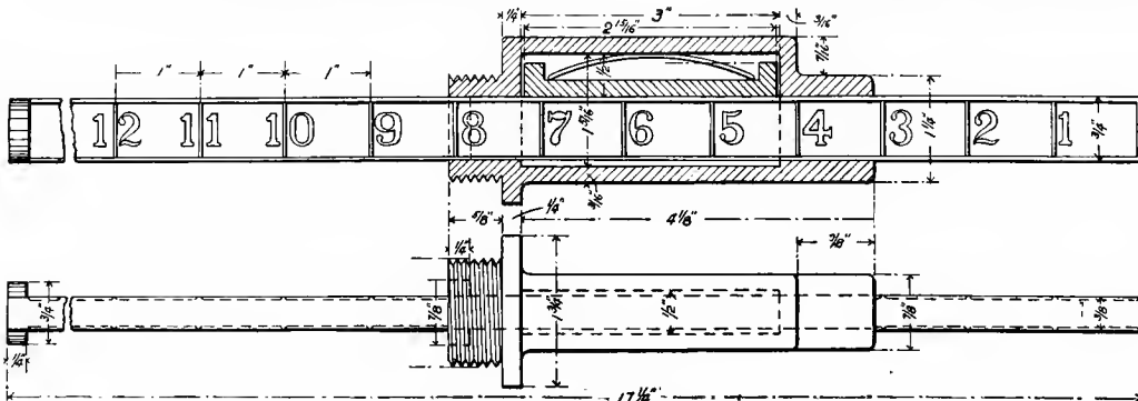
THE SCHROYER-THOMPSON PISTON-TRAVEL INDICATOR.
